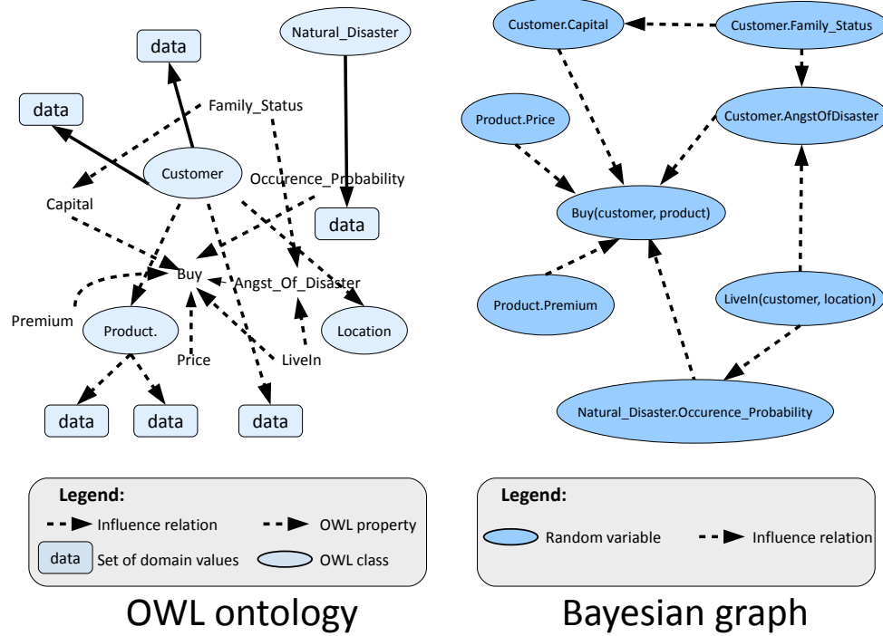
Figure 3.8: Ontobayes: Building a BN from an OWL ontology (insurance ontology)
