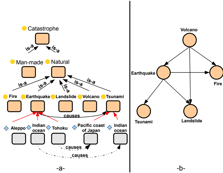
Figure 4.1: CBN-Ontology correspondances
