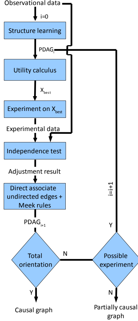
Figure 2.9: MYCADO Algorithm
