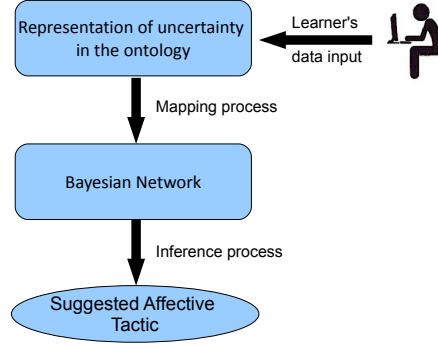
Figure 3.12: Mentor Model [71]
